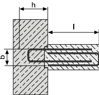
Type KS Console type for long cantilevers with separate inserted stirrup. Provided stirrup must be wired after bending-out operation
