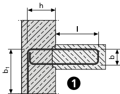
Type BK 1.) Console, closed stirrup, only for stirrup widths B = 90, 120, 140, 170 and 220 \text{ mm} possible
