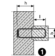
Type K 1.) Console, closed stirrup, only for stirrup widths B = 90, 120, 140, 170 and 220 \text{ mm} possible
